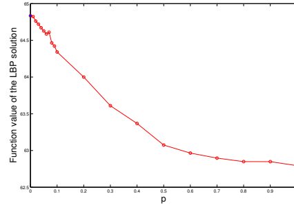
Figure 1: Value of the best solution found by max-LBP for different values of the rewiring probabilities.
